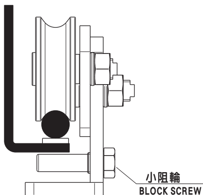
(1) 小阻輪 BLOCK SCREW
