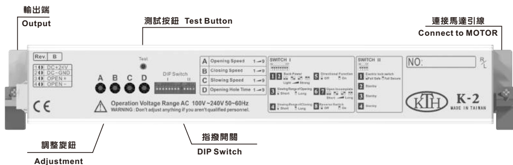
控制器面板圖 The FACEPLATE of MICRO-CONTROLLER
